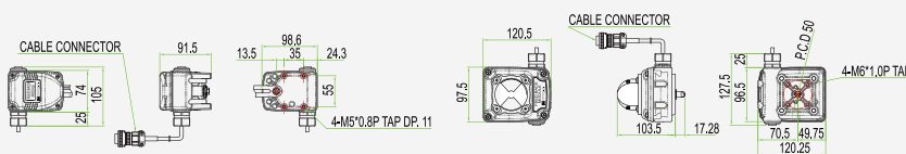
YT-3301L Sensor
